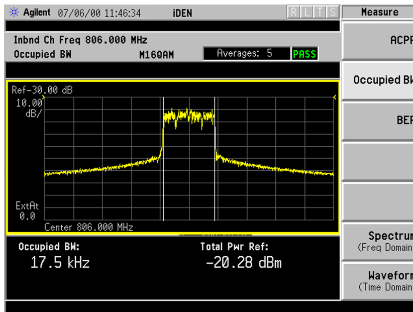
iDEN Occupied Bandwidth Measurement Results
