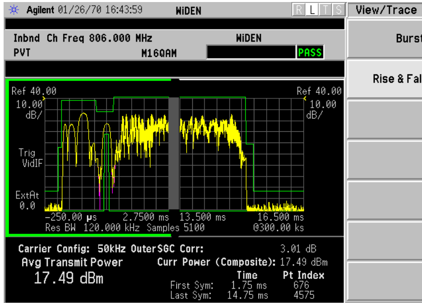
Figure 3-11 WiDEN Power vs. Time Result - Rise & Fall View
